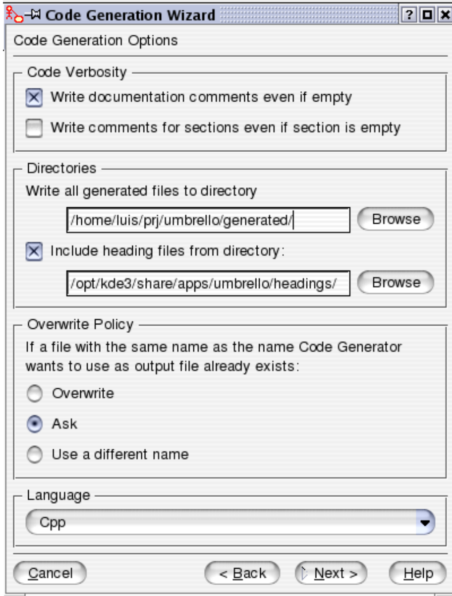
Options for the Code Generation in Umbrello UML Modeller
