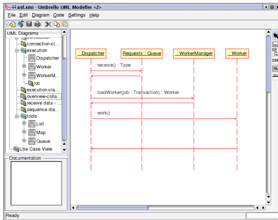
Umbrello UML Modeller showing a Sequence Diagram
