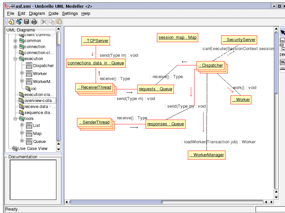
Umbrello UML Modeller showing a Collaboration Diagram
