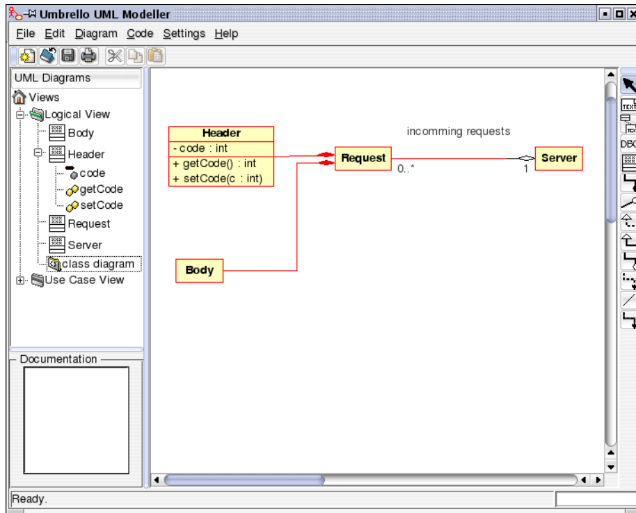
Umbrello UML Modeller showing a Class Diagram
