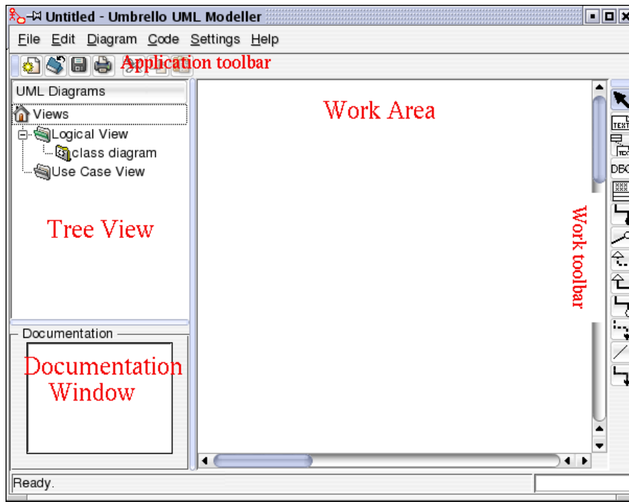
Umbrello UML Modeller's User Interface
