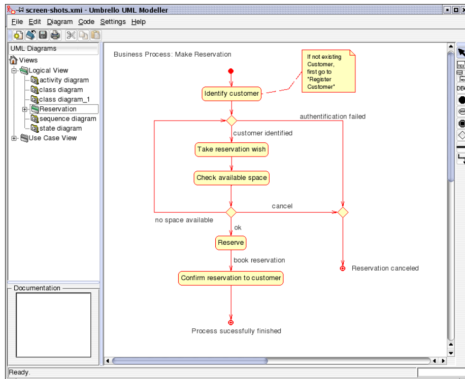
Umbrello UML Modeller showing an Activity Diagram
