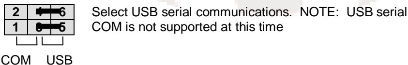
Figure 6: COM_SEL Option Header, JP5
